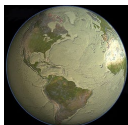
Trockene Erde (Credits: Cook, Nieman, USGS)
