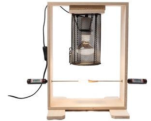
Experiment zur Albedo
